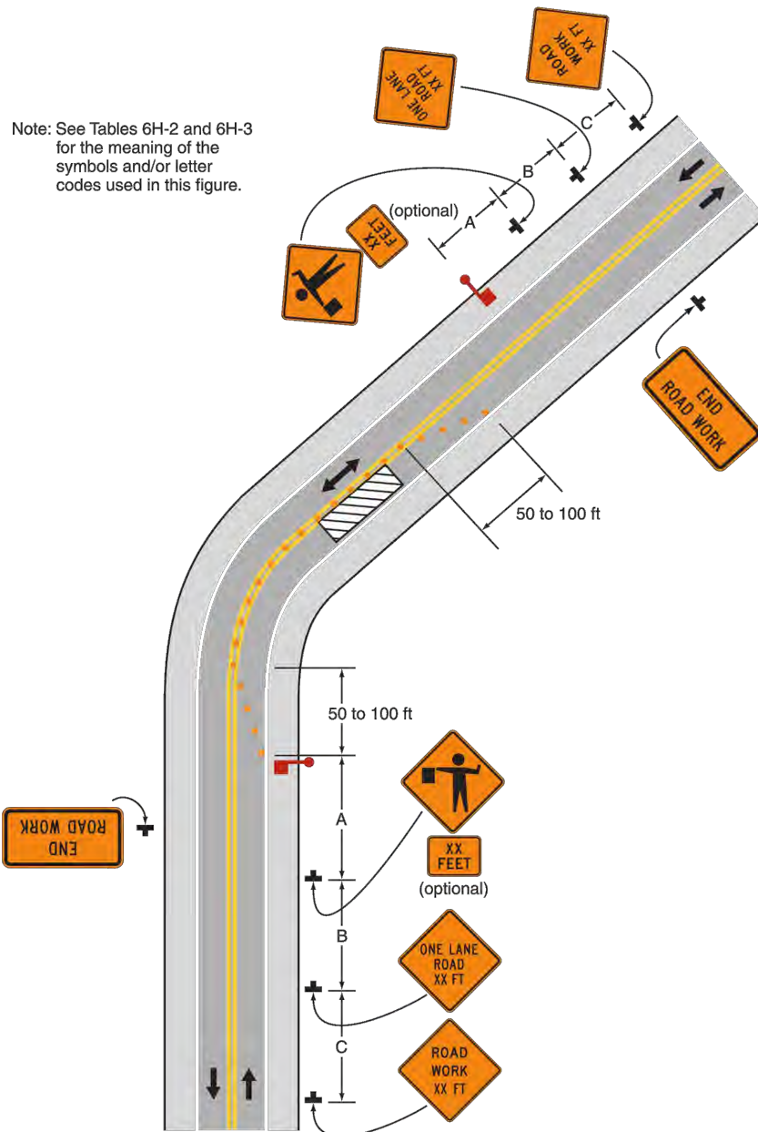
Typical Application 10
