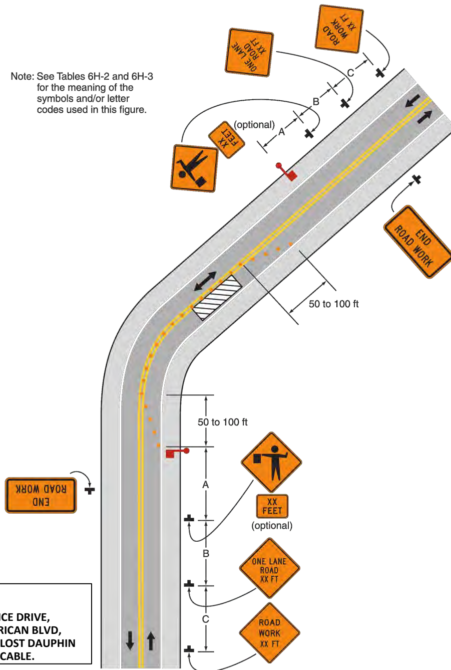
Typical Application 10
