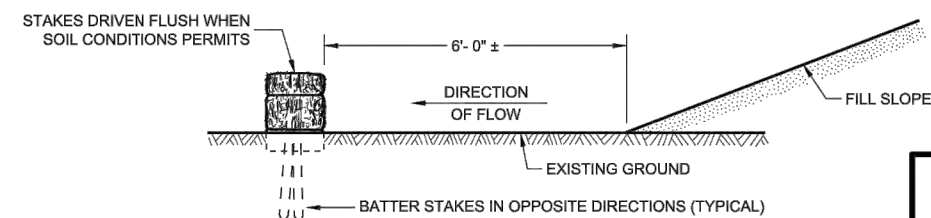
FRONT ELEVATION
