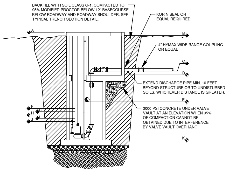
INTEGRAL VALVE VAULT SUBMERSIBLE LIFT STATION
