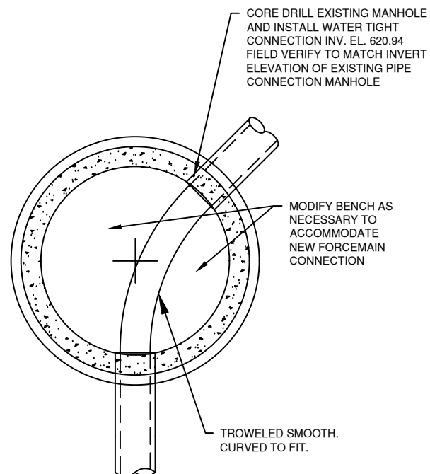
FORCEMAIN DISCHARGE MANHOLE CONNECTION
