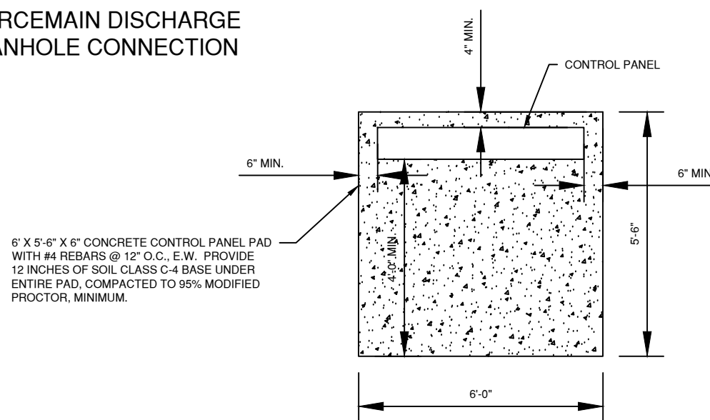
CONCRETE CONTROL PANEL PAD DETAIL
