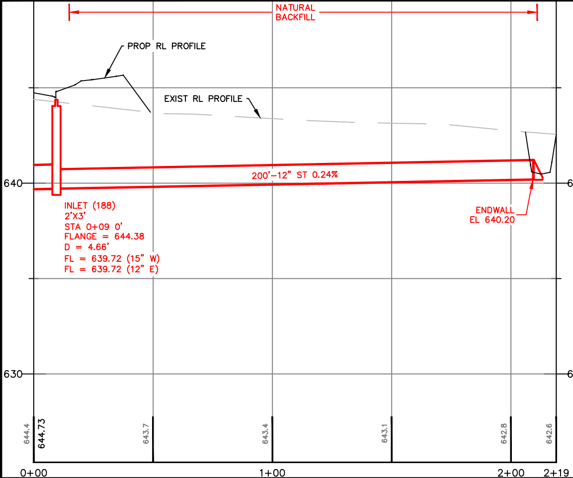
LOT 62 AND LOT 61 STORM SEWER
