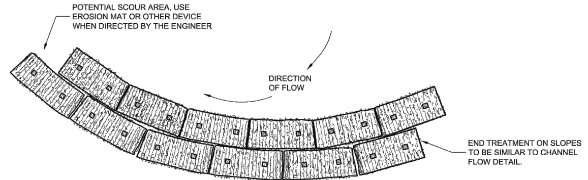
PLAN VIEW
