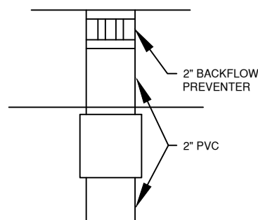
DRAIN DETAIL
