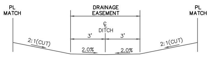
TYPICAL DITCH DETAIL
