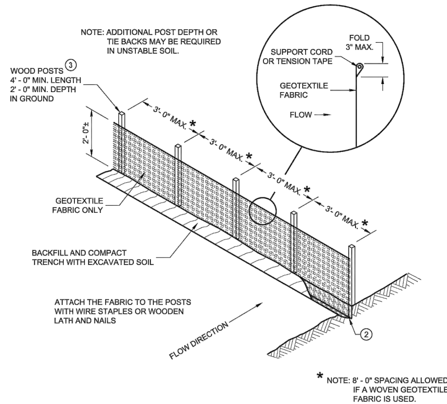
SILT FENCE
