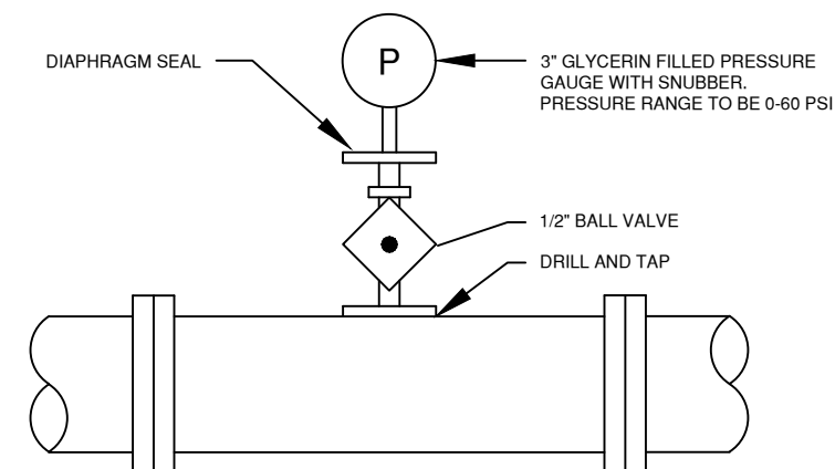
PRESSURE GAUGE DETAIL
