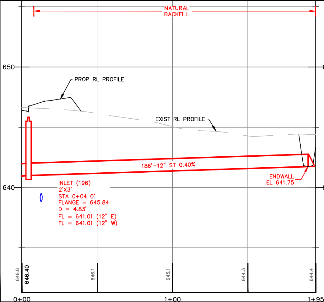
LOT 54 AND LOT 53 STORM SEWER
