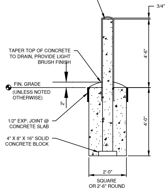
TYPICAL GUARD POST
