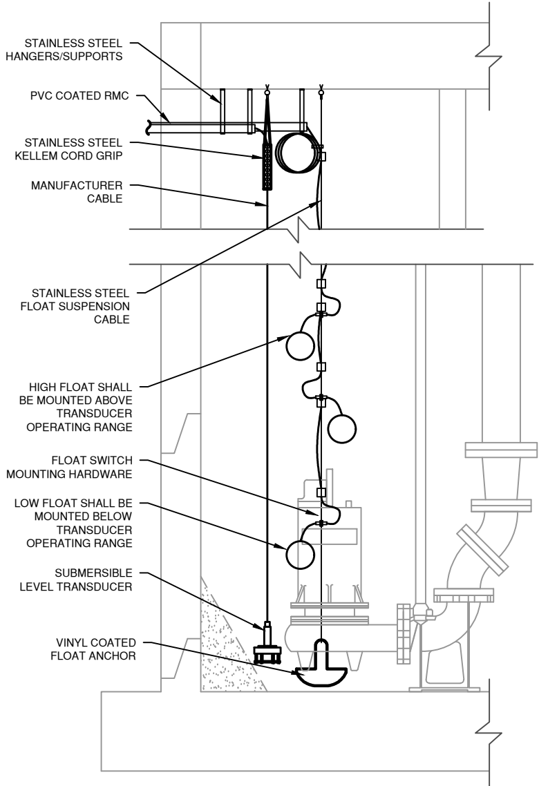
1 LEVEL SENSOR E501 INSTALL DETAIL SCALE: 1/2" = 1'-0"
