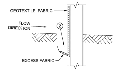
TRENCH DETAIL
