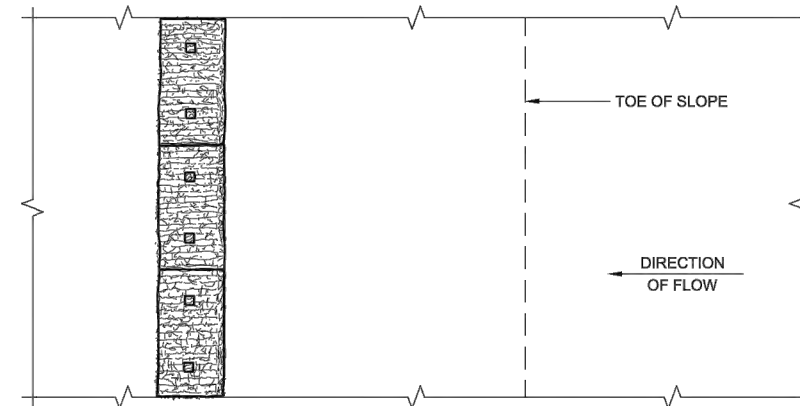
PLAN ELEVATION
