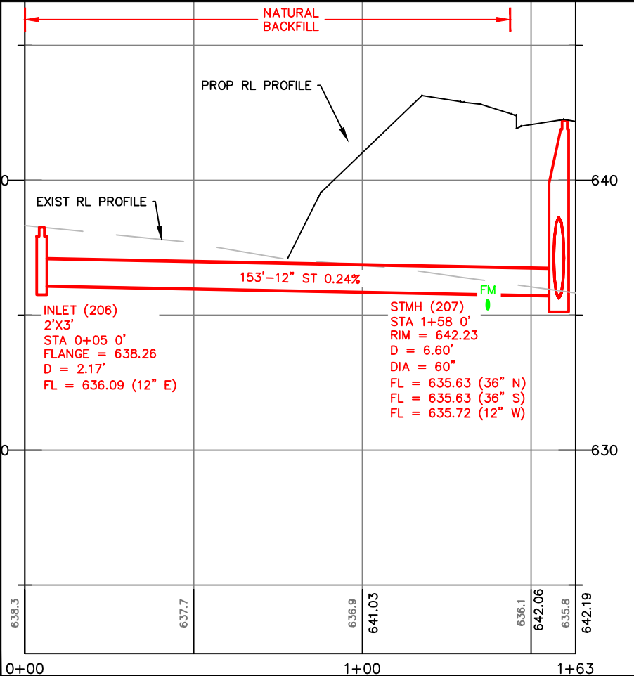
LOT 88 AND LOT 87 STORM SEWER
