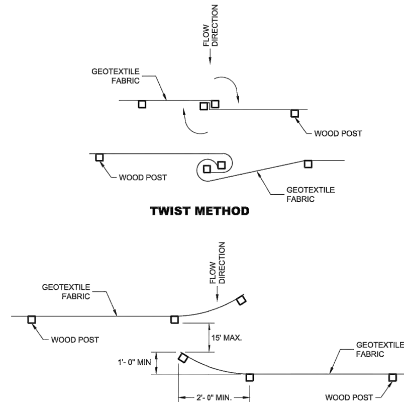
JOINING TWO LENGTHS OF SILT FENCE
