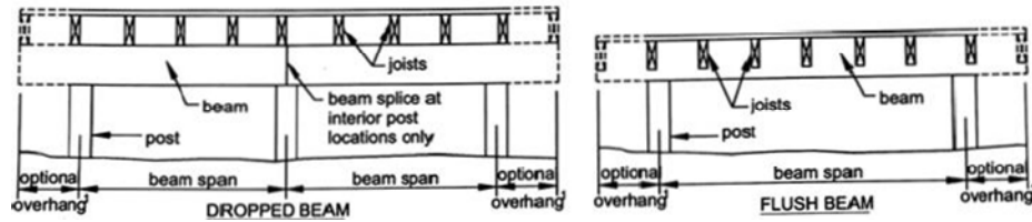
Figure 3 BEAM TYPES
