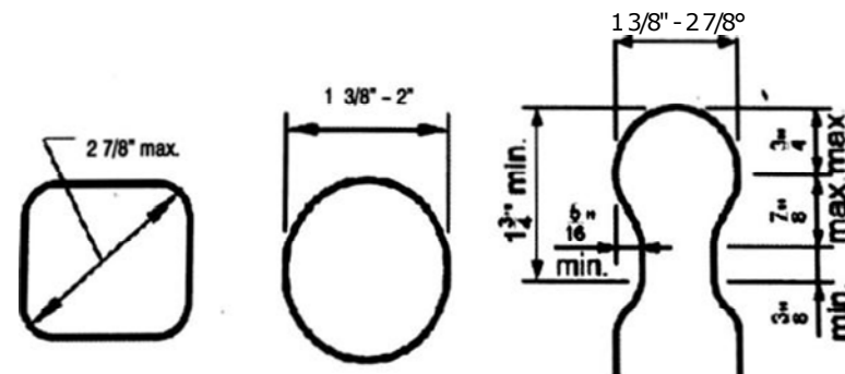
Figure 34 HANDRAIL GRASPABILITY
