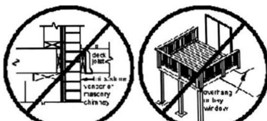
Figure 14 PROHIBITED LEDGER ATTACHMENTS
