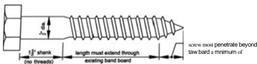
Figure 16 LAG SCREW
