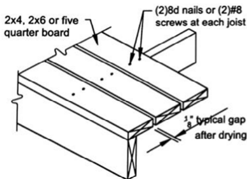
Figure 22 TYPICAL DECKING
