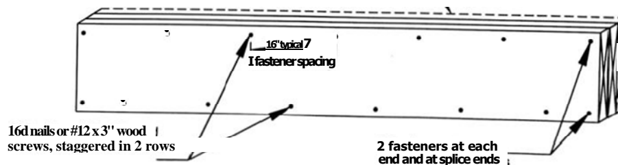
Figure 4 BEAM ASSEMBLY
