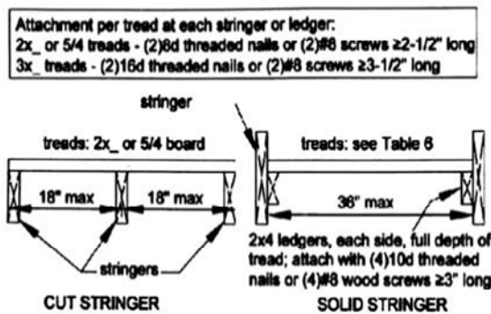
Figure 31 STAIRWAY TREADS
