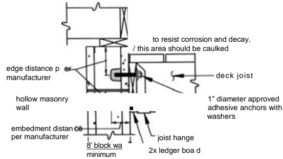
ATTACHMENT OF LEDGER BOARD TO HOLLOW FOUNDATION
