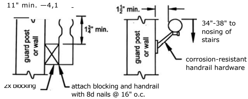
Figure 34 HANDRAIL GRASPABILITY
