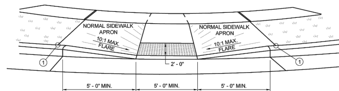
VIEW A - A FOR TYPE 1
