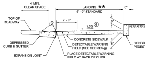
SECTION C - C FOR TYPE 1 - A
