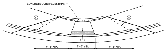
VIEW D - D FOR TYPE 1 - A
