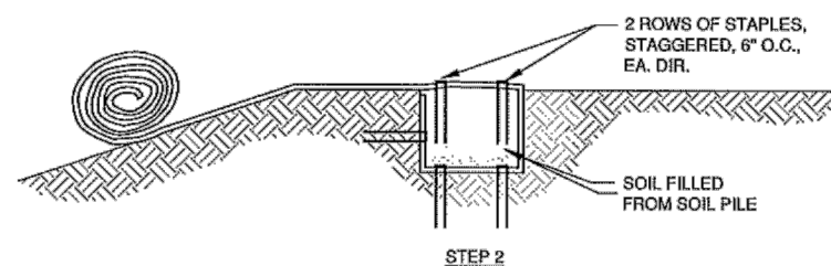
SLOPE TRENCHING METHOD "B"
