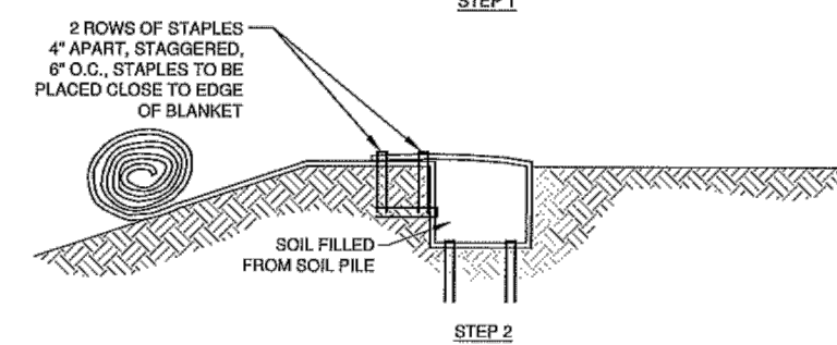
SLOPE TRENCHING METHOD "C"
