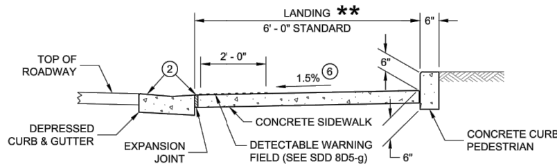
SECTION C - C FOR TYPE 1 - A
