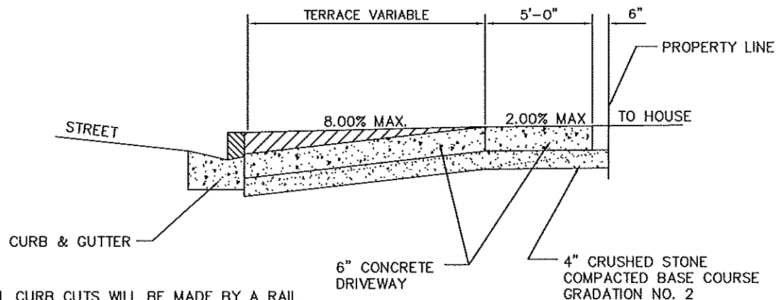
TYPICAL SECTION
