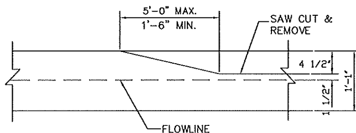
TYPICAL SECTION
