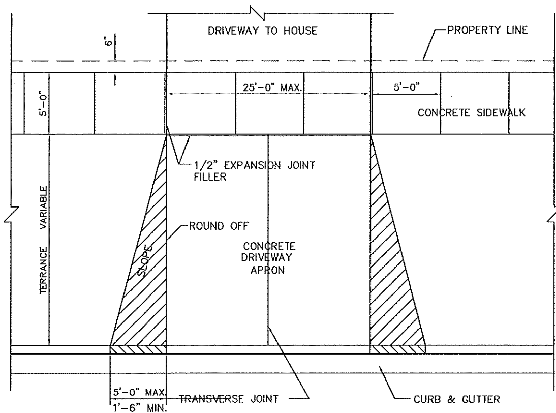
PLAN VIEW
